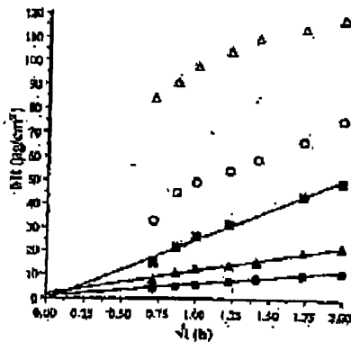
Figure 3—Effect of drug loading in the PIB adhesives on the release profiles of fentanyl into an aqueous buffer sink at 32 °C: 1% (●), 2% (▲), 4% (■), 5% (○), 8% (△). The initial burst effect was observed for those adhesive matrices with drug loading above 4%.
